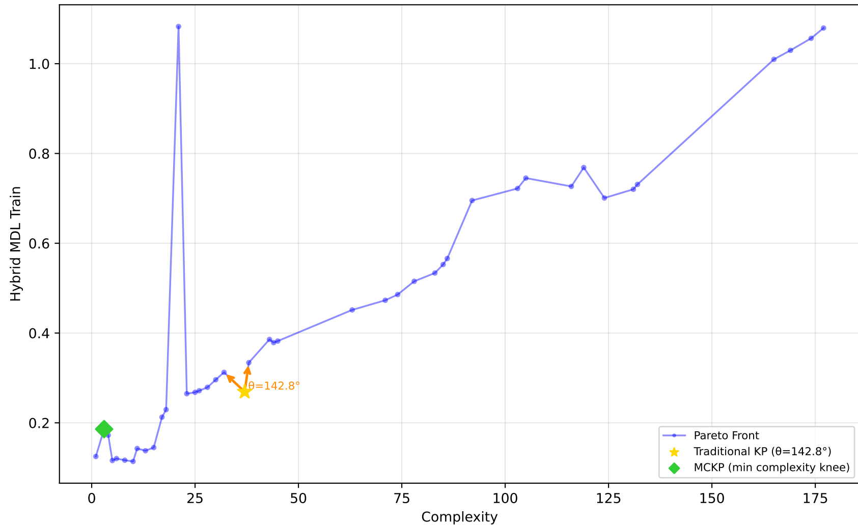
712_chscase_geyser1 - Run 14 - SVP - Hybrid MDL Train \lambda_1=1.00, \lambda_2=1.00, \lambda_3=0.00 | Difficulty: 0.76 | Method: hmr
