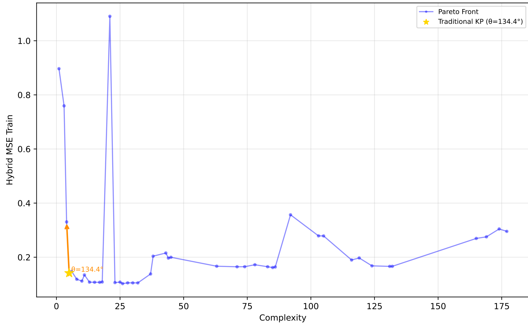
712_chscase_geyser1 - Run 14 - SVP - Hybrid MSE Train \lambda_1=0.00, \lambda_2=1.00, \lambda_3=1.00 | Difficulty: 0.76 | Method: hmr
