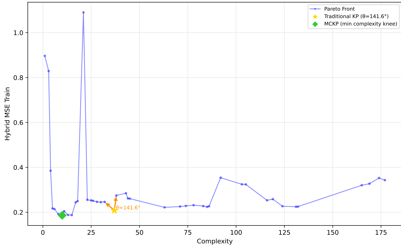
712_chscase_geyser1 - Run 14 - SVP - Hybrid MSE Train \lambda_1=1.00, \lambda_2=1.00, \lambda_3=0.00 | Difficulty: 0.76 | Method: hmr
