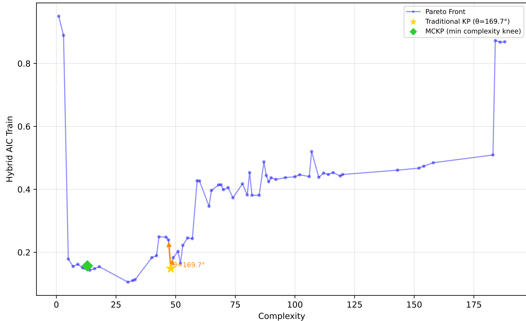
712_chscase_geyser1 - Run 15 - MVP - Hybrid AIC Train \lambda_1=0.20, \lambda_2=1.00, \lambda_3=1.00 | Difficulty: 0.40 | Method: mckp
