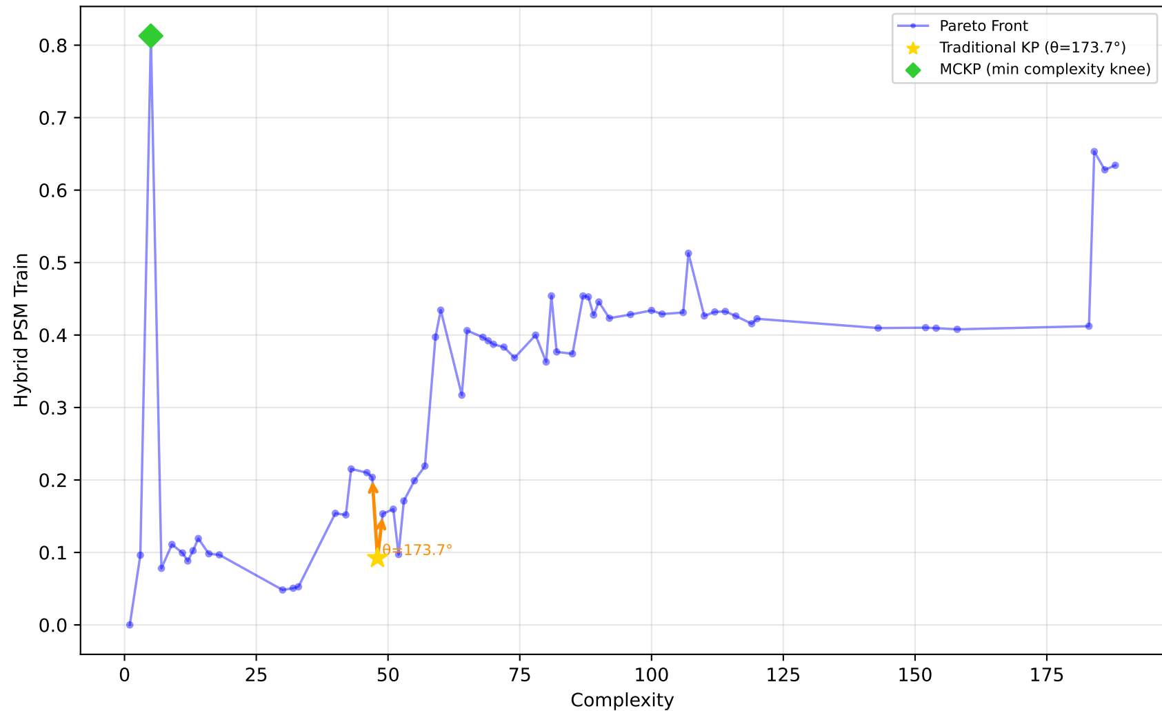
712_chscase_geyser1 - Run 15 - MVP - Hybrid PSM Train \lambda_1=0.20, \lambda_2=1.00, \lambda_3=1.00 | Difficulty: 0.40 | Method: mckp
