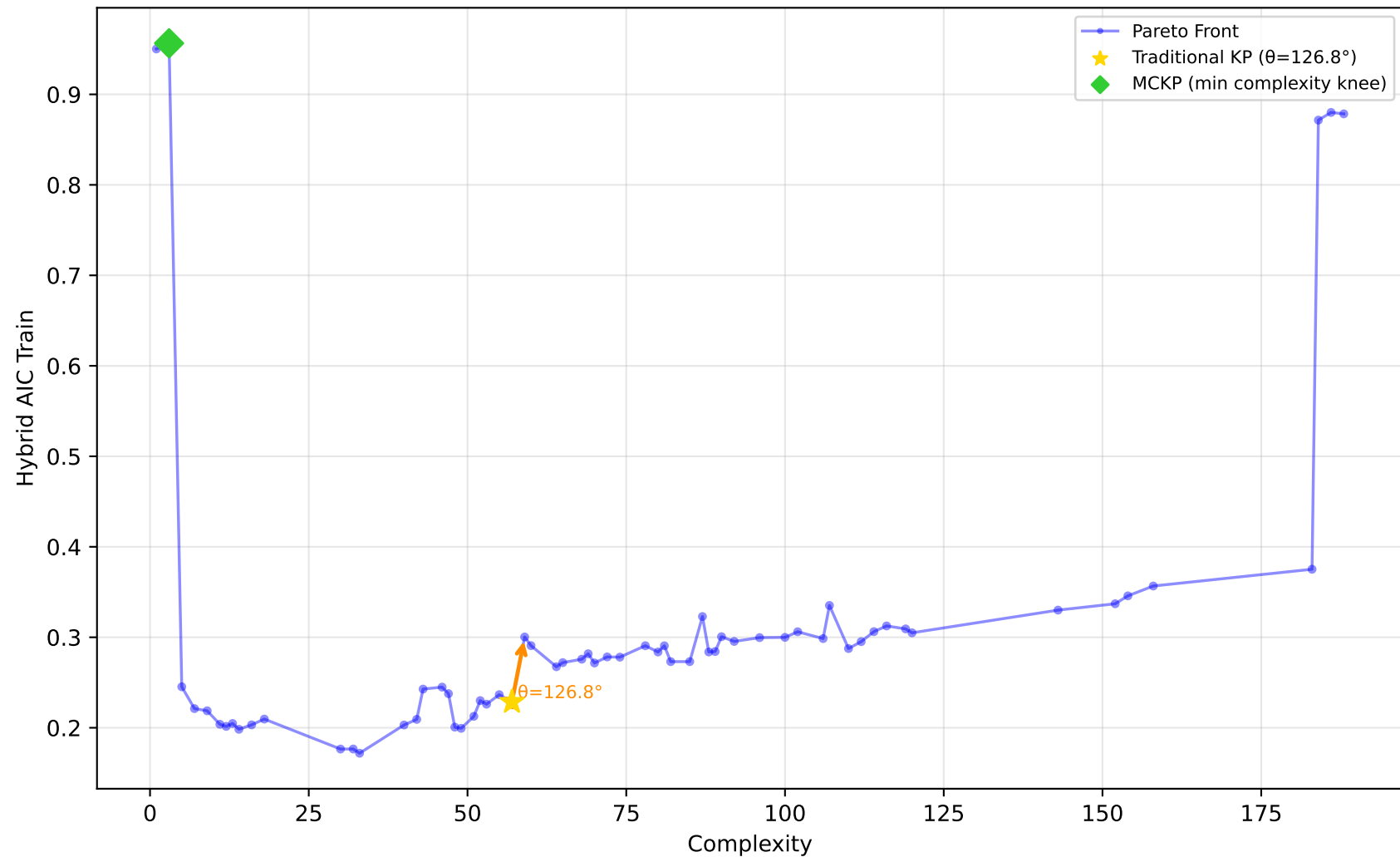
712_chscase_geyser1 - Run 15 - SVP - Hybrid AIC Train \lambda_1=1.00, \lambda_2=1.00, \lambda_3=0.00 | Difficulty: 0.40 | Method: mckp
