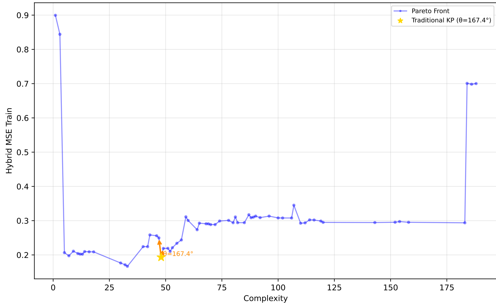
712_chscase_geyser1 - Run 15 - SVP - Hybrid MSE Train \lambda_1=1.00, \lambda_2=1.00, \lambda_3=0.00 | Difficulty: 0.40 | Method: mckp
