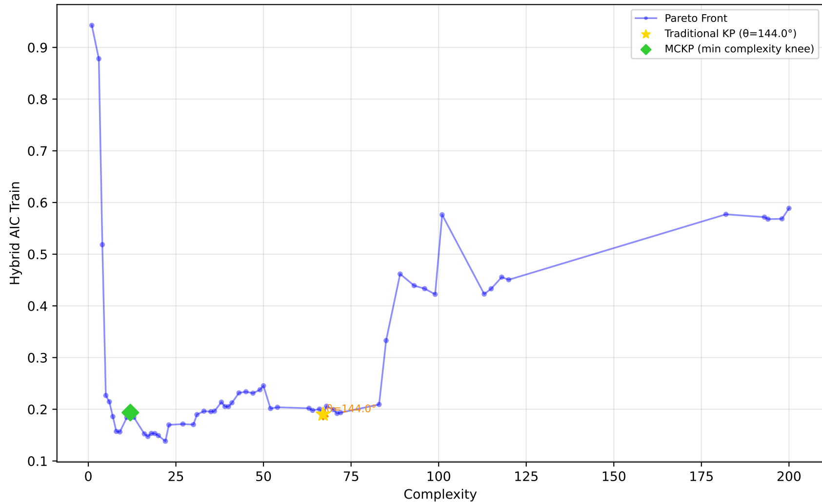
712_chscase_geyser1 - Run 16 - MVP - Hybrid AIC Train \lambda_1=0.20, \lambda_2=1.00, \lambda_3=1.00 | Difficulty: 1.00 | Method: hmr
