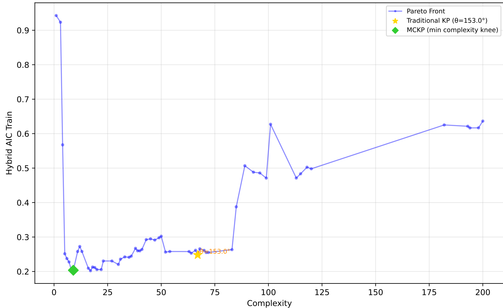
712_chscase_geyser1 - Run 16 - MVP - Hybrid AIC Train \lambda_1=1.00, \lambda_2=1.00, \lambda_3=1.00 | Difficulty: 1.00 | Method: hmr
