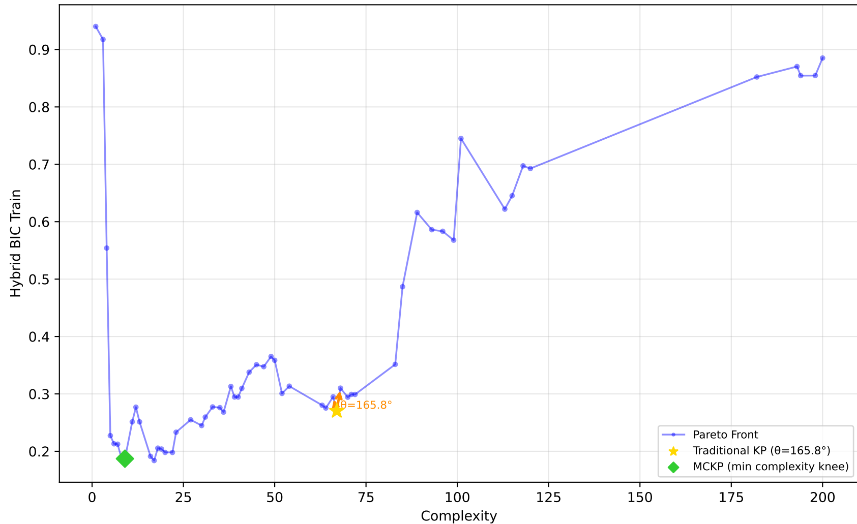
712_chscase_geyser1 - Run 16 - MVP - Hybrid BIC Train \lambda_1=1.00, \lambda_2=1.00, \lambda_3=1.00 | Difficulty: 1.00 | Method: hmr
