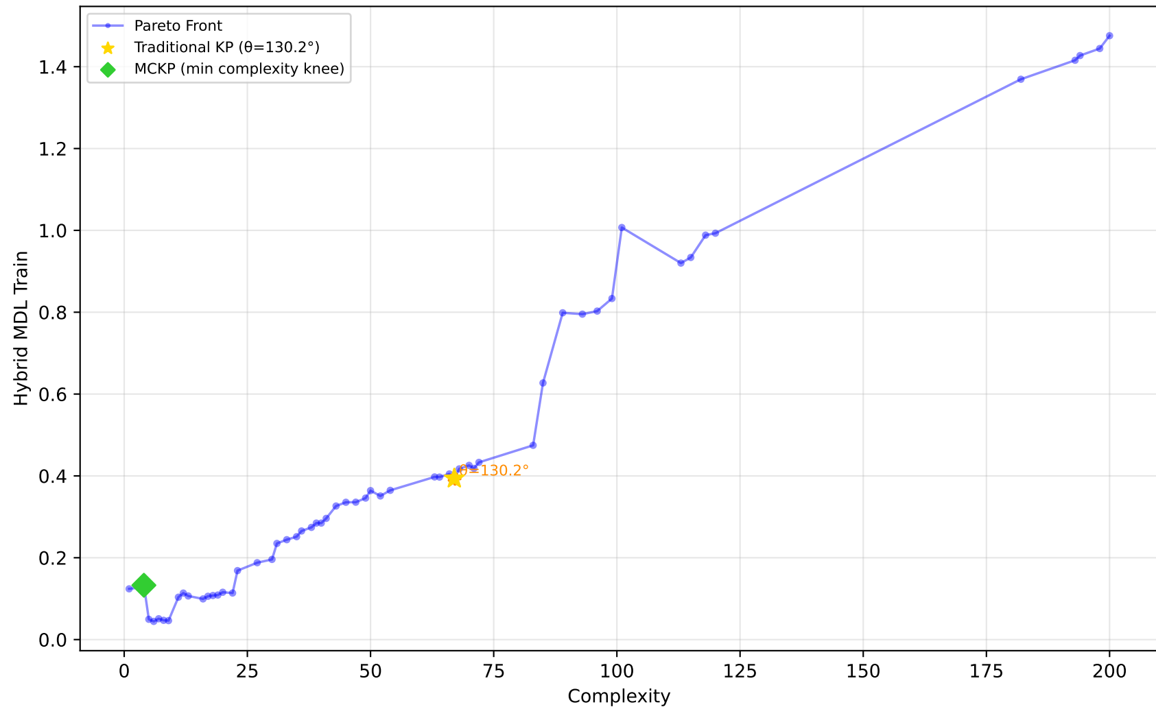
712_chscase_geyser1 - Run 16 - MVP - Hybrid MDL Train \lambda_1=0.20, \lambda_2=1.00, \lambda_3=1.00 | Difficulty: 1.00 | Method: hmr
