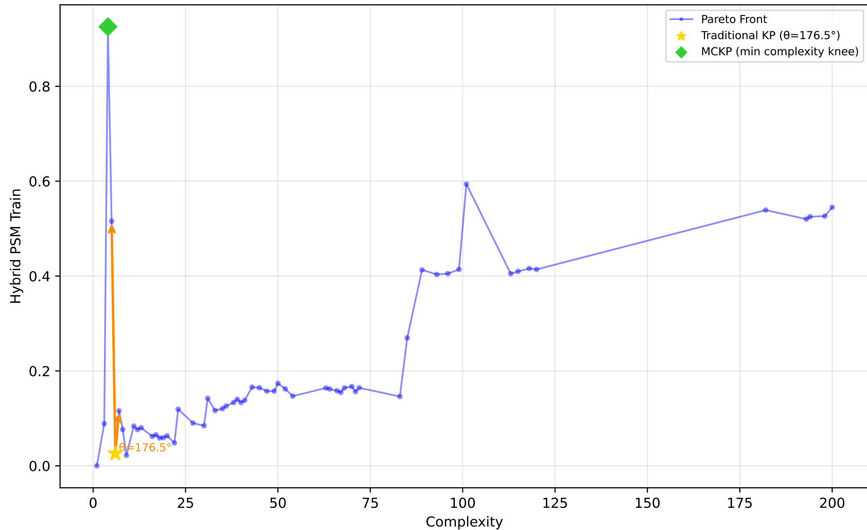
712_chscase_geyser1 - Run 16 - MVP - Hybrid PSM Train \lambda_1=0.20, \lambda_2=1.00, \lambda_3=1.00 | Difficulty: 1.00 | Method: hmr
