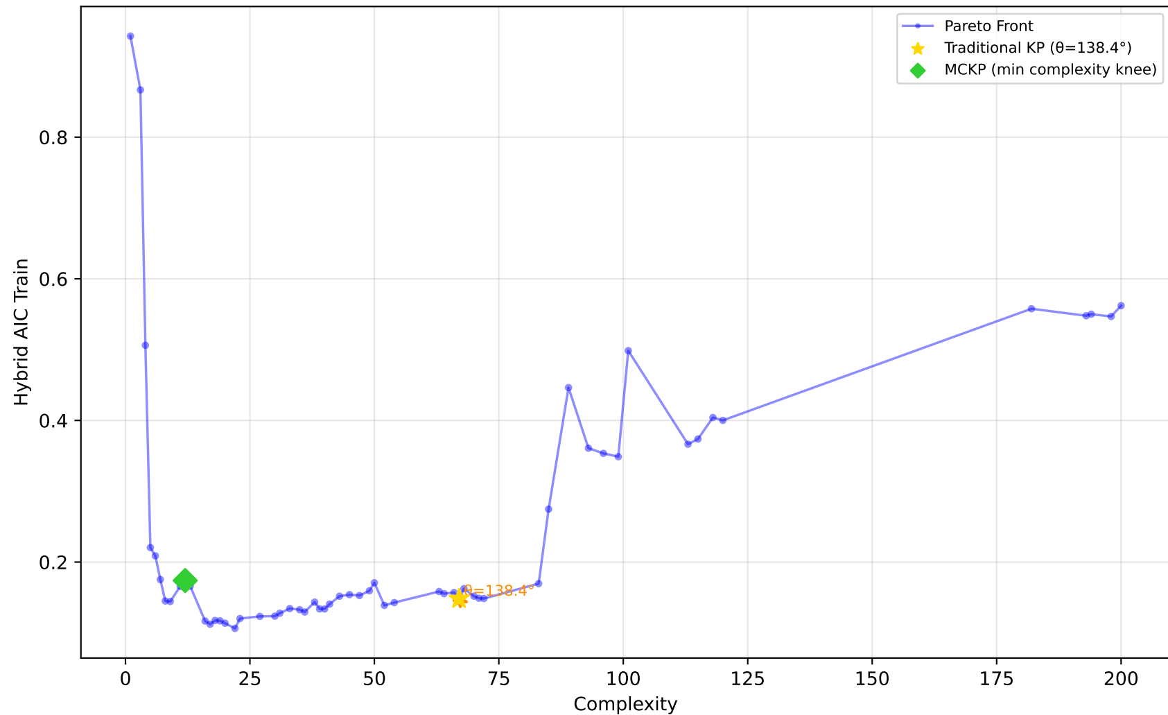
712_chscase_geyser1 - Run 16 - SVP - Hybrid AIC Train \lambda_1=0.00 , \lambda_2=1.00 , \lambda_3=1.00 | Difficulty: 1.00 | Method: hmr
