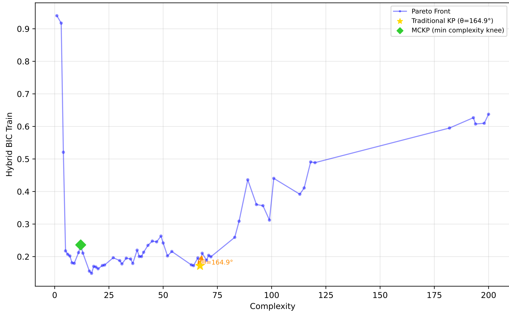
712_chscase_geyser1 - Run 16 - SVP - Hybrid BIC Train \lambda_1=1.00, \lambda_2=1.00, \lambda_3=0.00 | Difficulty: 1.00 | Method: hmr
