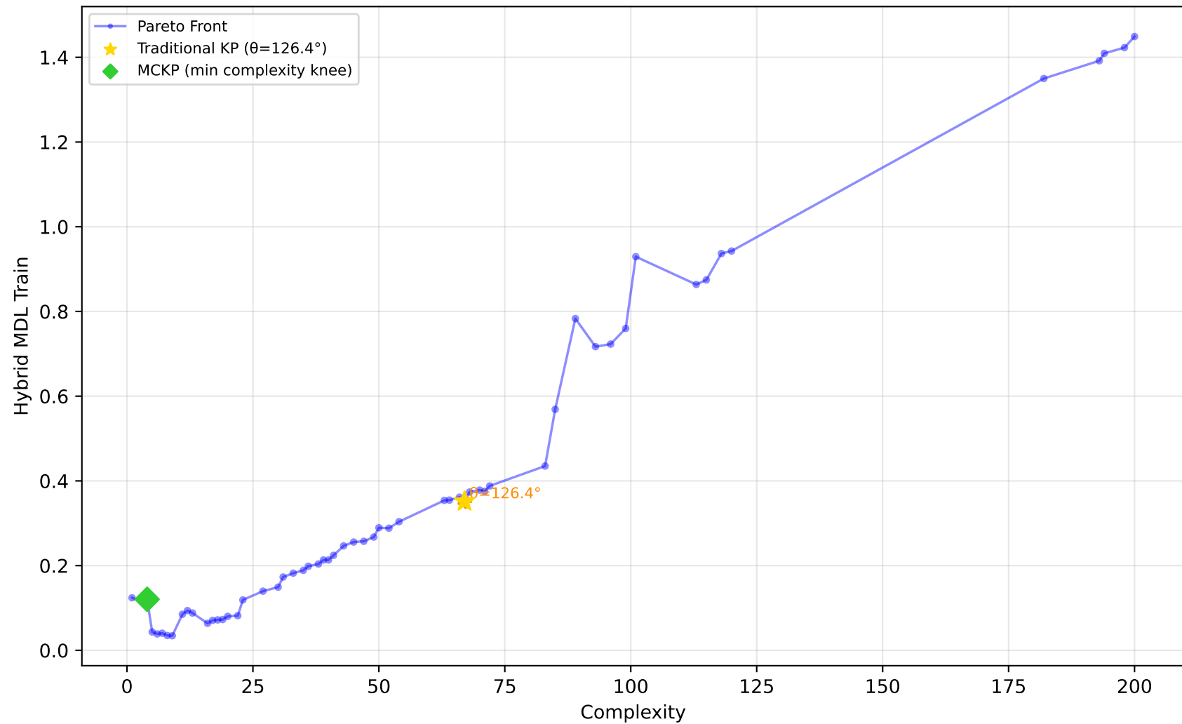
712_chscase_geyser1 - Run 16 - SVP - Hybrid MDL Train \lambda_1=0.00, \lambda_2=1.00, \lambda_3=1.00 | Difficulty: 1.00 | Method: hmr
