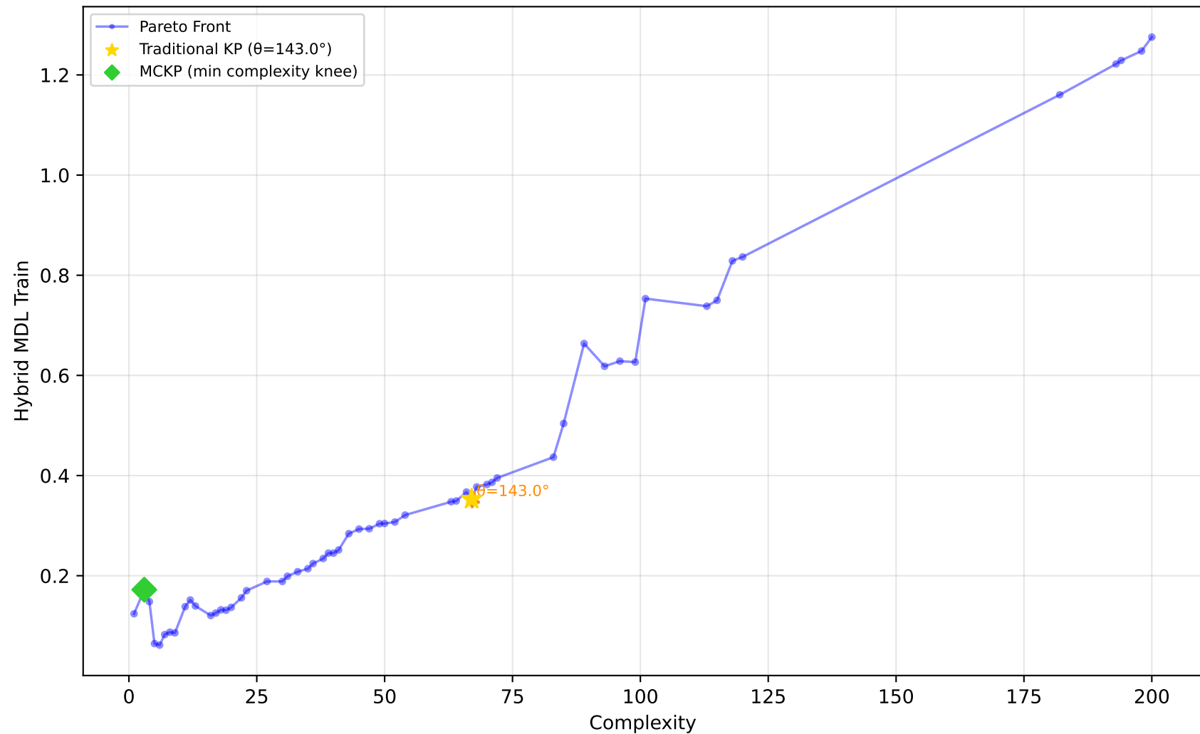
712_chscase_geyser1 - Run 16 - SVP - Hybrid MDL Train \lambda_1=1.00, \lambda_2=1.00, \lambda_3=0.00 | Difficulty: 1.00 | Method: hmr
