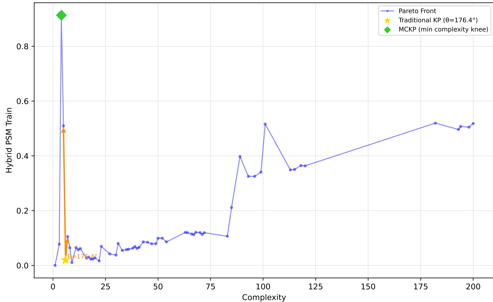
712_chscase_geyser1 - Run 16 - SVP - Hybrid PSM Train \lambda_1=0.00, \lambda_2=1.00, \lambda_3=1.00 | Difficulty: 1.00 | Method: hmr
