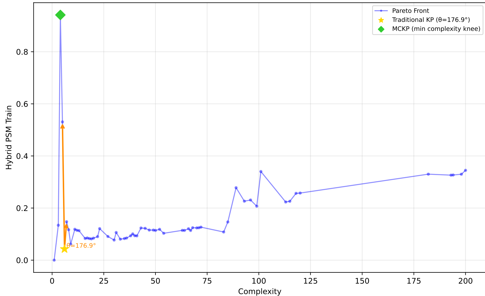
712_chscase_geyser1 - Run 16 - SVP - Hybrid PSM Train \lambda_1=1.00, \lambda_2=1.00, \lambda_3=0.00 | Difficulty: 1.00 | Method: hmr
