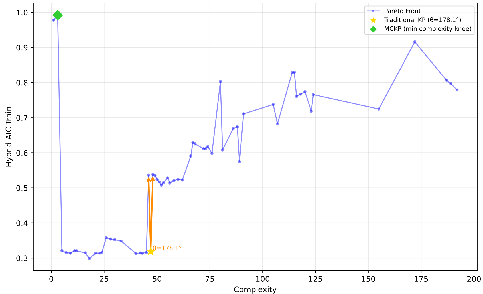
712_chscase_geyser1 - Run 17 - MVP - Hybrid AIC Train \lambda_1=1.00, \lambda_2=1.00, \lambda_3=1.00 | Difficulty: 0.41 | Method: mckp
