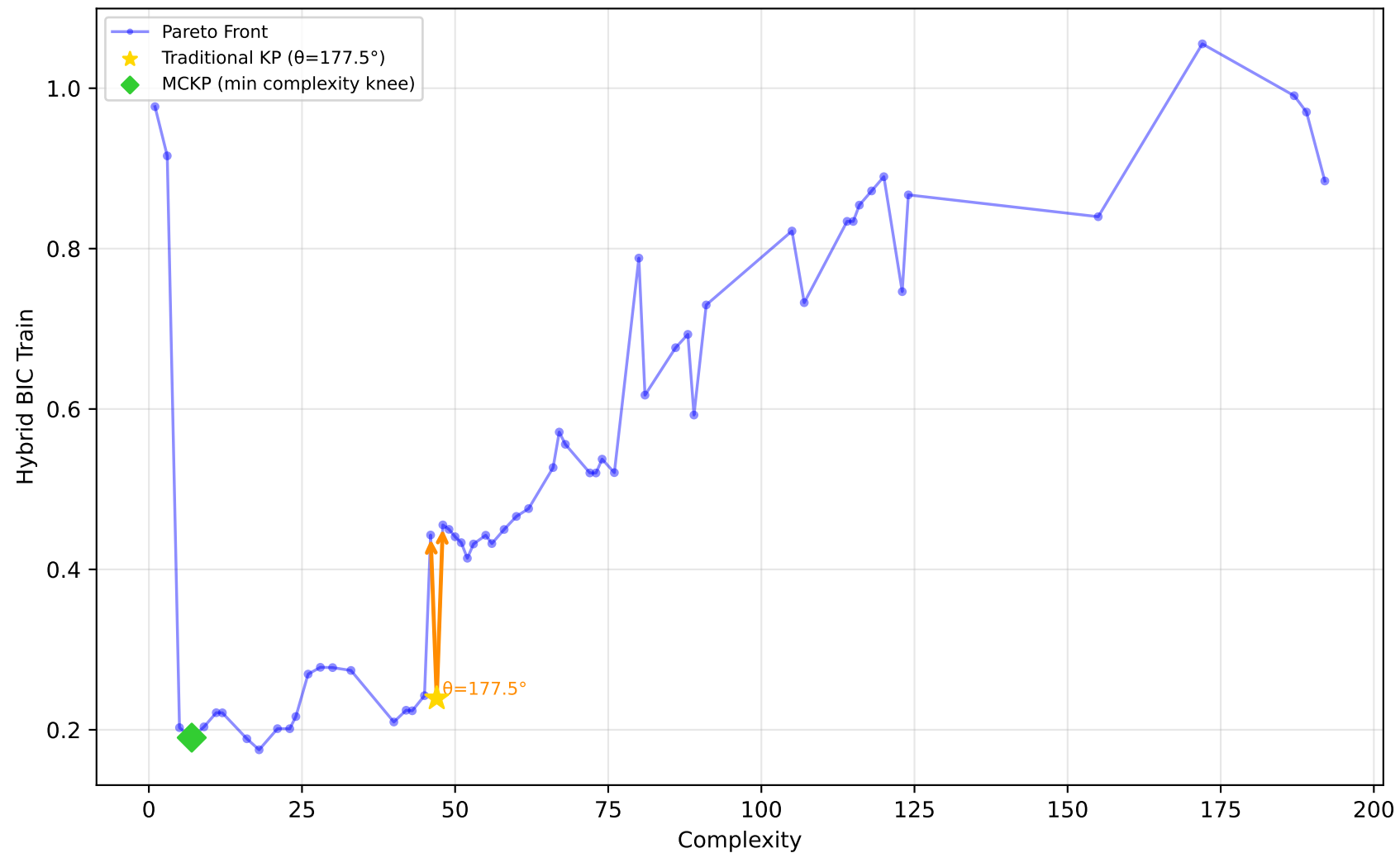
712_chscase_geyser1 - Run 17 - MVP - Hybrid BIC Train \lambda_1=0.20, \lambda_2=1.00, \lambda_3=1.00 | Difficulty: 0.41 | Method: mckp
