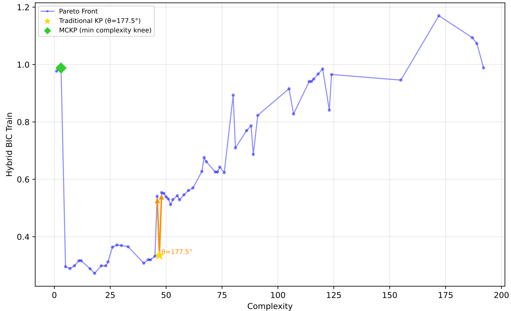
712_chscase_geyser1 - Run 17 - MVP - Hybrid BIC Train \lambda_1=1.00, \lambda_2=1.00, \lambda_3=1.00 | Difficulty: 0.41 | Method: mckp
