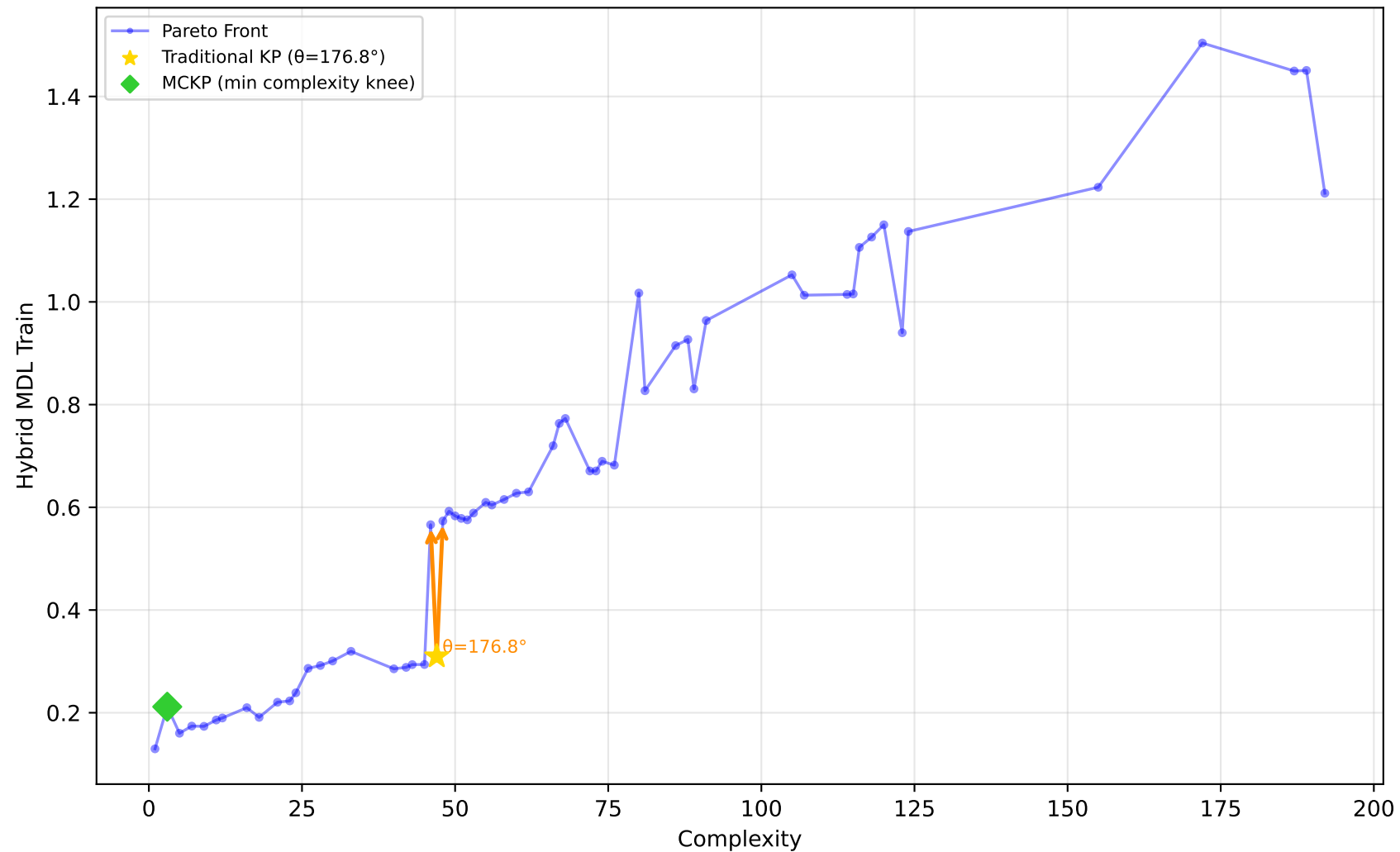
712_chscase_geyser1 - Run 17 - MVP - Hybrid MDL Train \lambda_1=1.00, \lambda_2=1.00, \lambda_3=1.00 | Difficulty: 0.41 | Method: mckp
