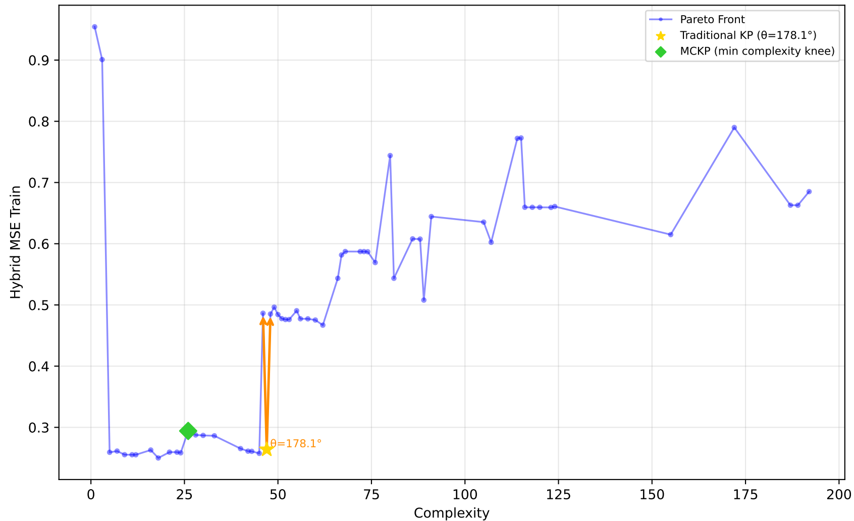
712_chscase_geyser1 - Run 17 - MVP - Hybrid MSE Train \lambda_1=1.00, \lambda_2=1.00, \lambda_3=1.00 | Difficulty: 0.41 | Method: mckp
