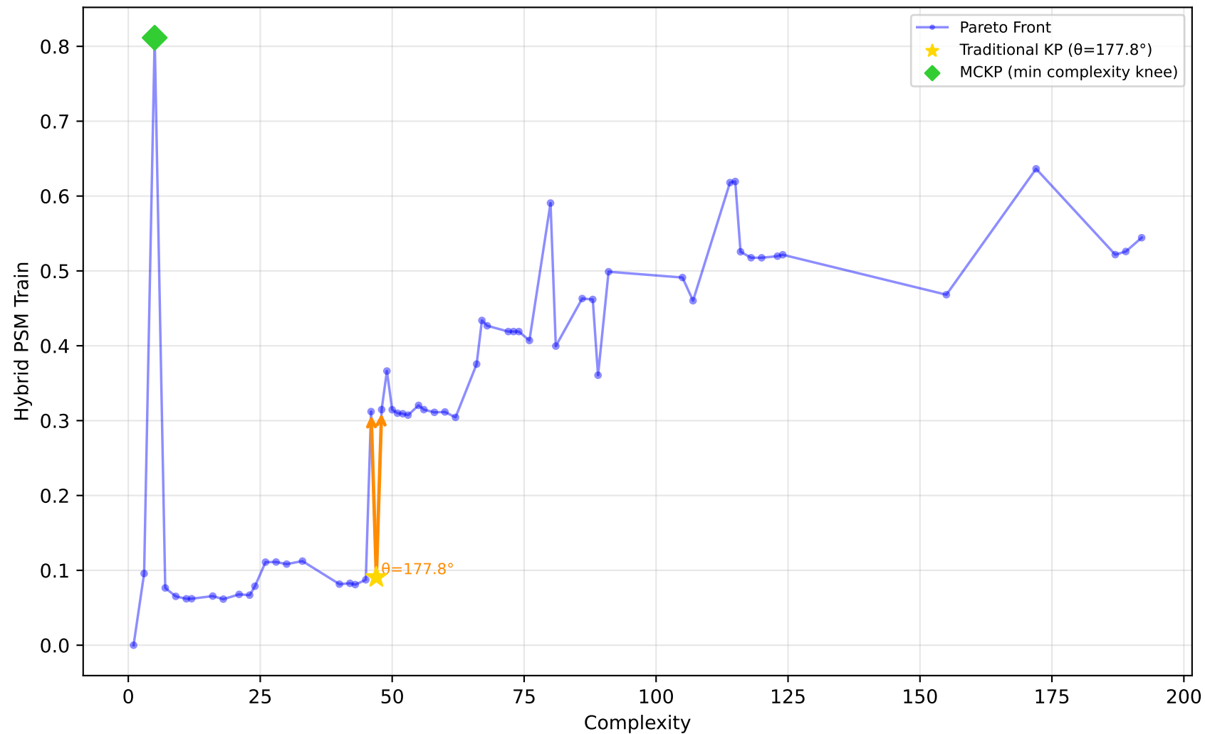
712_chscase_geyser1 - Run 17 - MVP - Hybrid PSM Train \lambda_1=0.20, \lambda_2=1.00, \lambda_3=1.00 | Difficulty: 0.41 | Method: mckp
