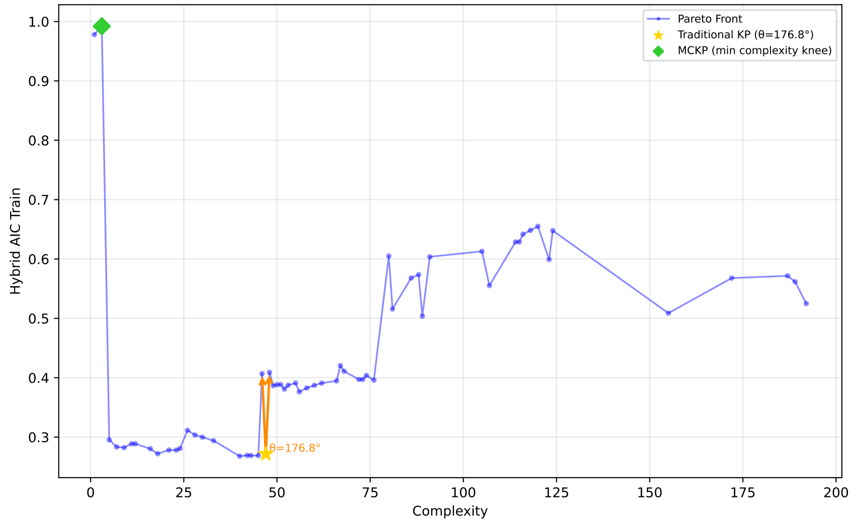
712_chscase_geyser1 - Run 17 - SVP - Hybrid AIC Train \lambda_1=1.00, \lambda_2=1.00, \lambda_3=0.00 | Difficulty: 0.41 | Method: mckp
