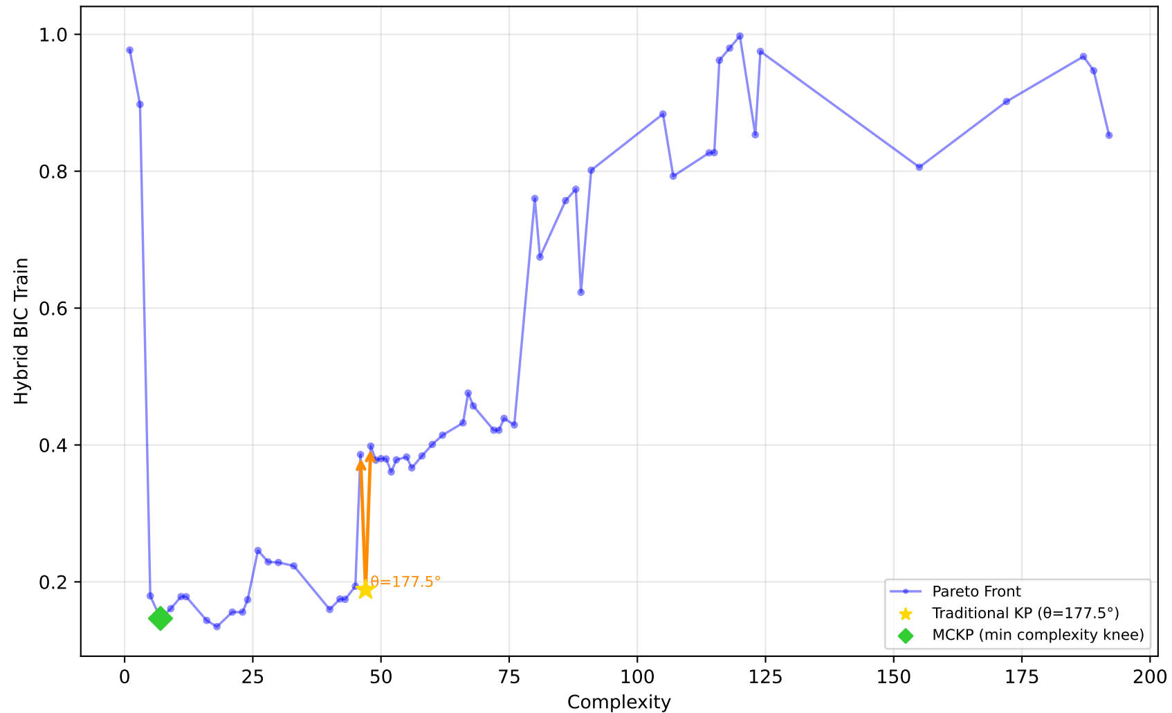
712_chscase_geyser1 - Run 17 - SVP - Hybrid BIC Train \lambda_1=0.00, \lambda_2=1.00, \lambda_3=1.00 | Difficulty: 0.41 | Method: mckp
