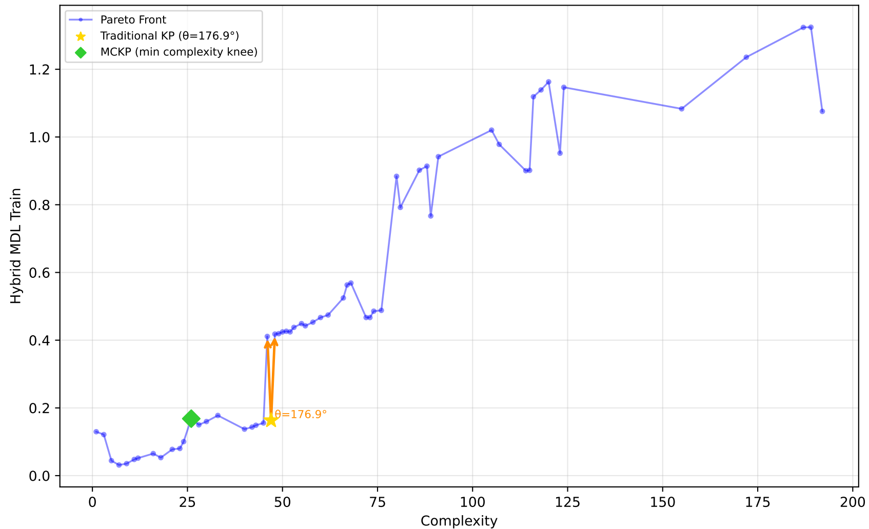
712_chscase_geyser1 - Run 17 - SVP - Hybrid MDL Train \lambda_1=0.00, \lambda_2=1.00, \lambda_3=1.00 | Difficulty: 0.41 | Method: mckp
