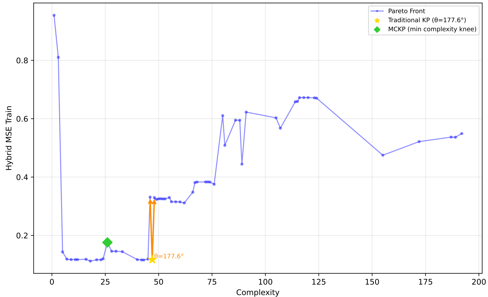
712_chscase_geyser1 - Run 17 - SVP - Hybrid MSE Train \lambda_1=0.00, \lambda_2=1.00, \lambda_3=1.00 | Difficulty: 0.41 | Method: mckp
