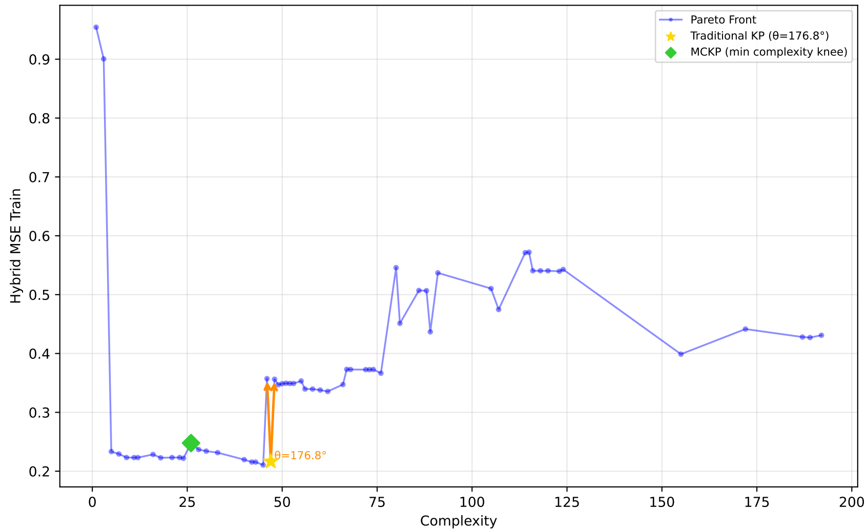
712_chscase_geyser1 - Run 17 - SVP - Hybrid MSE Train \lambda_1=1.00, \lambda_2=1.00, \lambda_3=0.00 | Difficulty: 0.41 | Method: mckp
