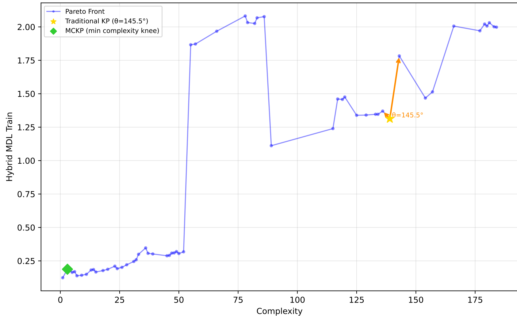
712_chscase_geyser1 - Run 18 - MVP - Hybrid MDL Train \lambda_1=1.00 , \lambda_2=1.00 , \lambda_3=1.00 | Difficulty: 0.64 | Method: hmr
