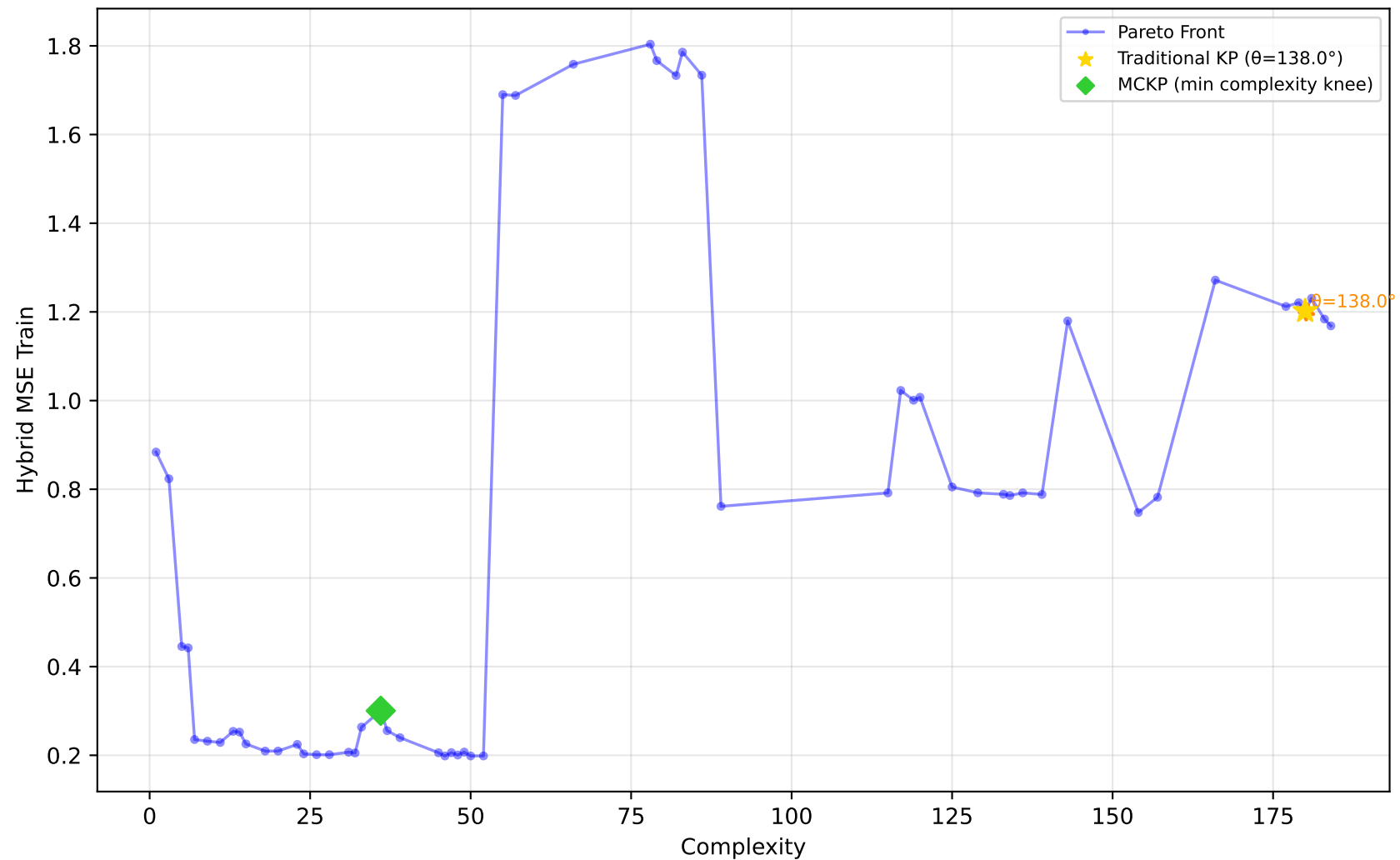
712_chscase_geyser1 - Run 18 - MVP - Hybrid MSE Train \lambda_1=1.00, \lambda_2=1.00, \lambda_3=1.00 | Difficulty: 0.64 | Method: hmr
