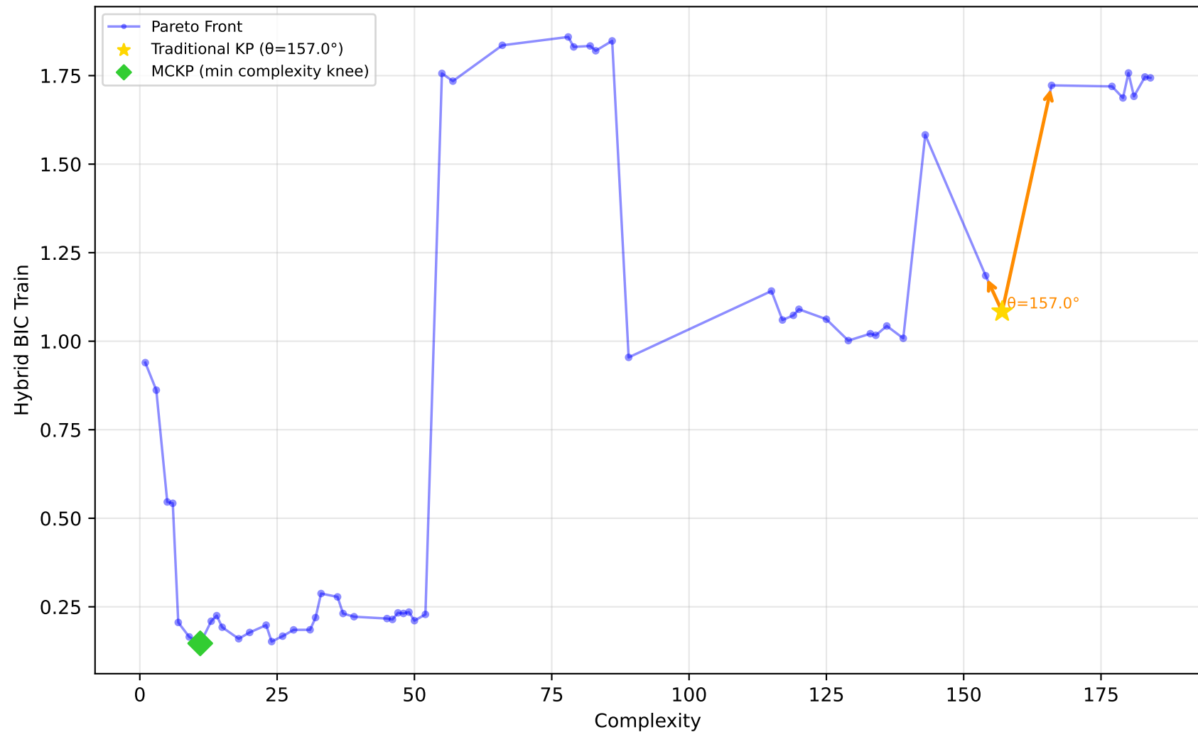
712_chscase_geyser1 - Run 18 - SVP - Hybrid BIC Train \lambda_1=0.00 , \lambda_2=1.00 , \lambda_3=1.00 | Difficulty: 0.64 | Method: hmr
