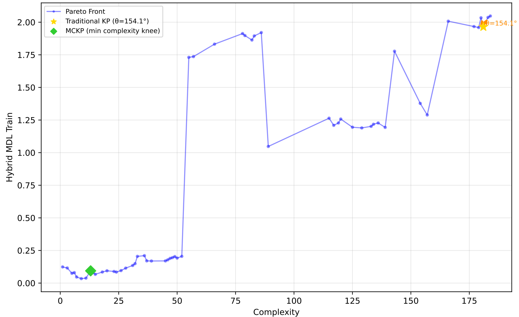
712_chscase_geyser1 - Run 18 - SVP - Hybrid MDL Train \lambda_1=0.00, \lambda_2=1.00, \lambda_3=1.00 | Difficulty: 0.64 | Method: hmr
