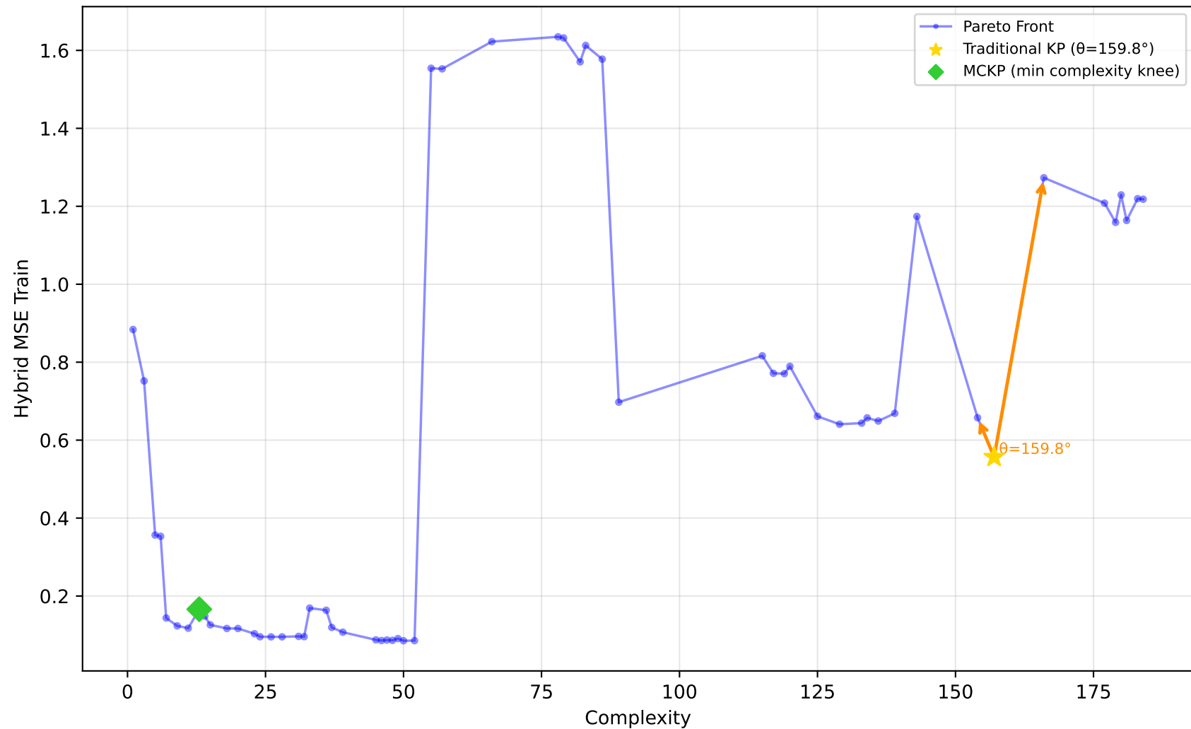
712_chscase_geyser1 - Run 18 - SVP - Hybrid MSE Train \lambda_1=0.00, \lambda_2=1.00, \lambda_3=1.00 | Difficulty: 0.64 | Method: hmr
