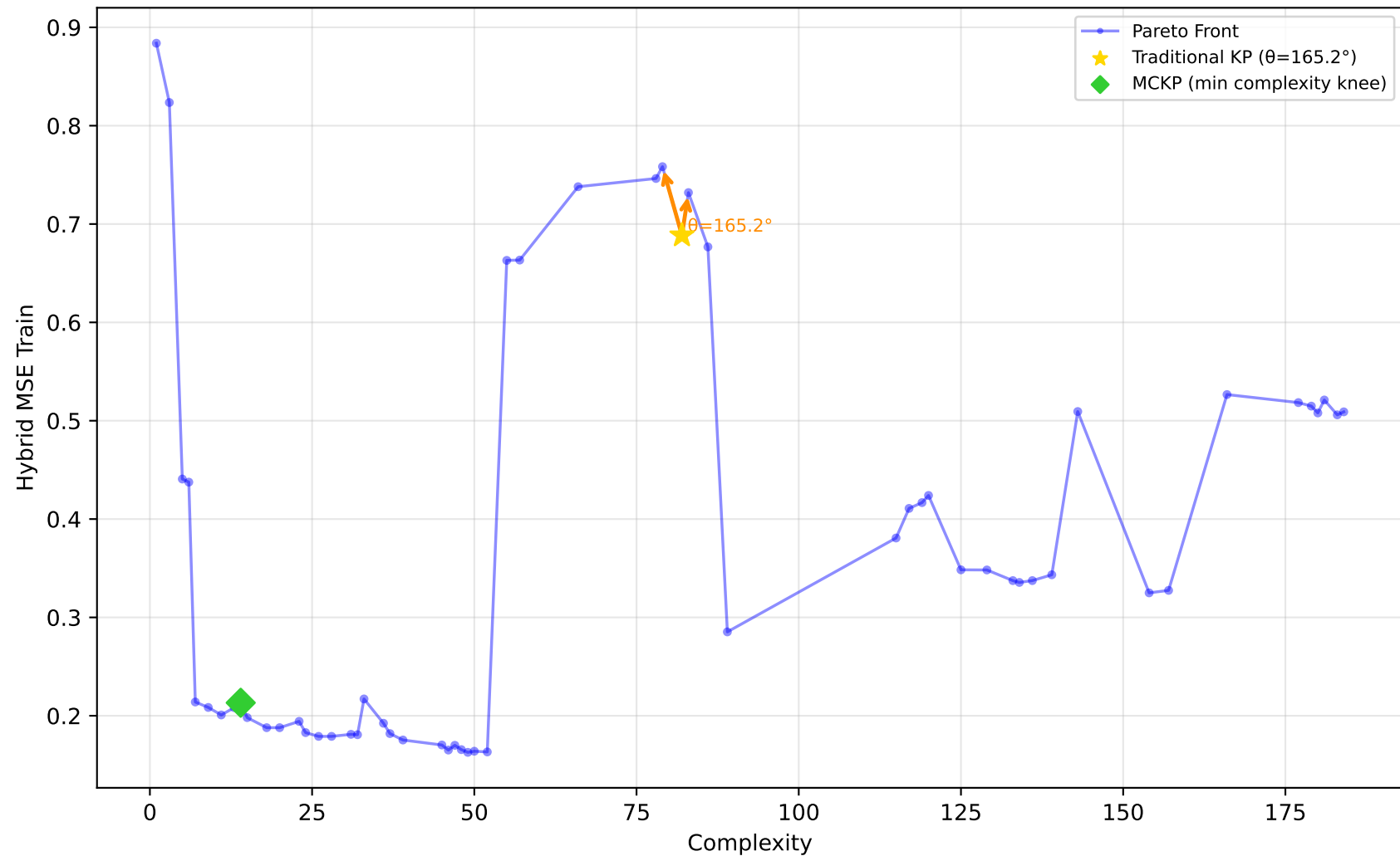
712_chscase_geyser1 - Run 18 - SVP - Hybrid MSE Train \lambda_1=1.00, \lambda_2=1.00, \lambda_3=0.00 | Difficulty: 0.64 | Method: hmr
