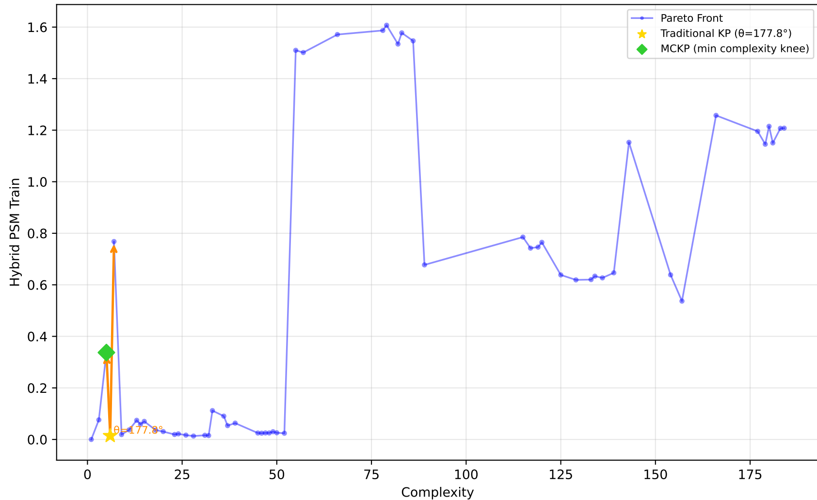
712_chscase_geyser1 - Run 18 - SVP - Hybrid PSM Train \lambda_1=0.00, \lambda_2=1.00, \lambda_3=1.00 | Difficulty: 0.64 | Method: hmr
