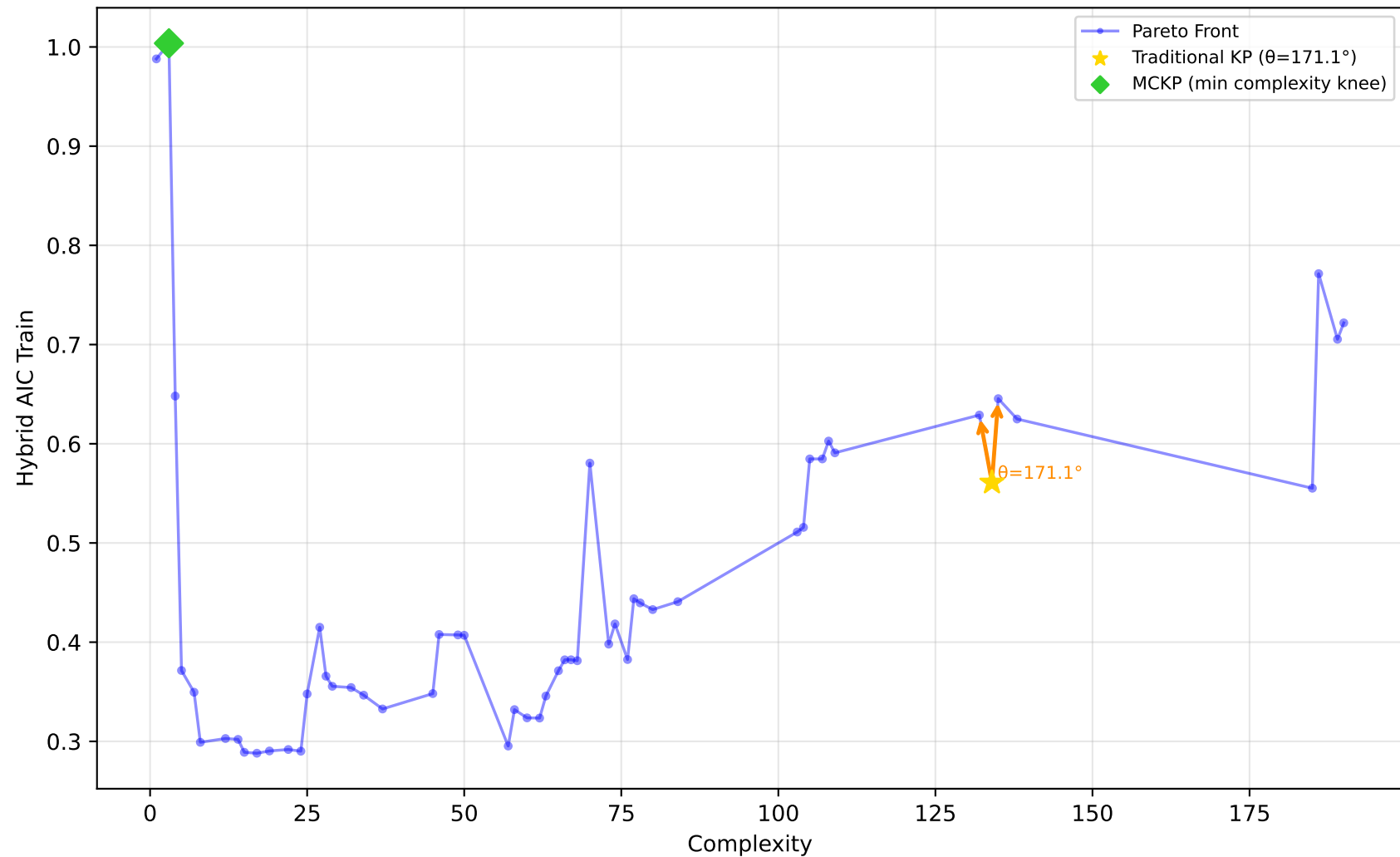
712_chscase_geyser1 - Run 19 - MVP - Hybrid AIC Train \lambda_1=1.00, \lambda_2=1.00, \lambda_3=1.00 | Difficulty: 0.58 | Method: mckp
