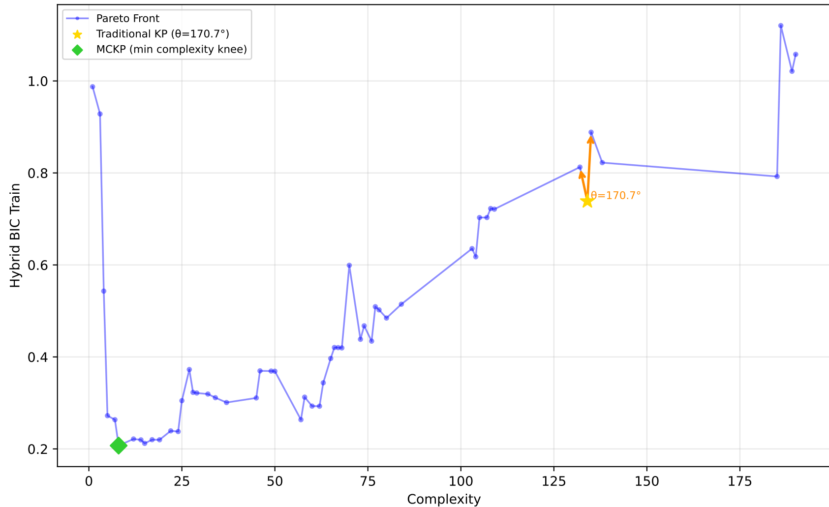
712_chscase_geyser1 - Run 19 - MVP - Hybrid BIC Train \lambda_1=0.20, \lambda_2=1.00, \lambda_3=1.00 | Difficulty: 0.58 | Method: mckp
