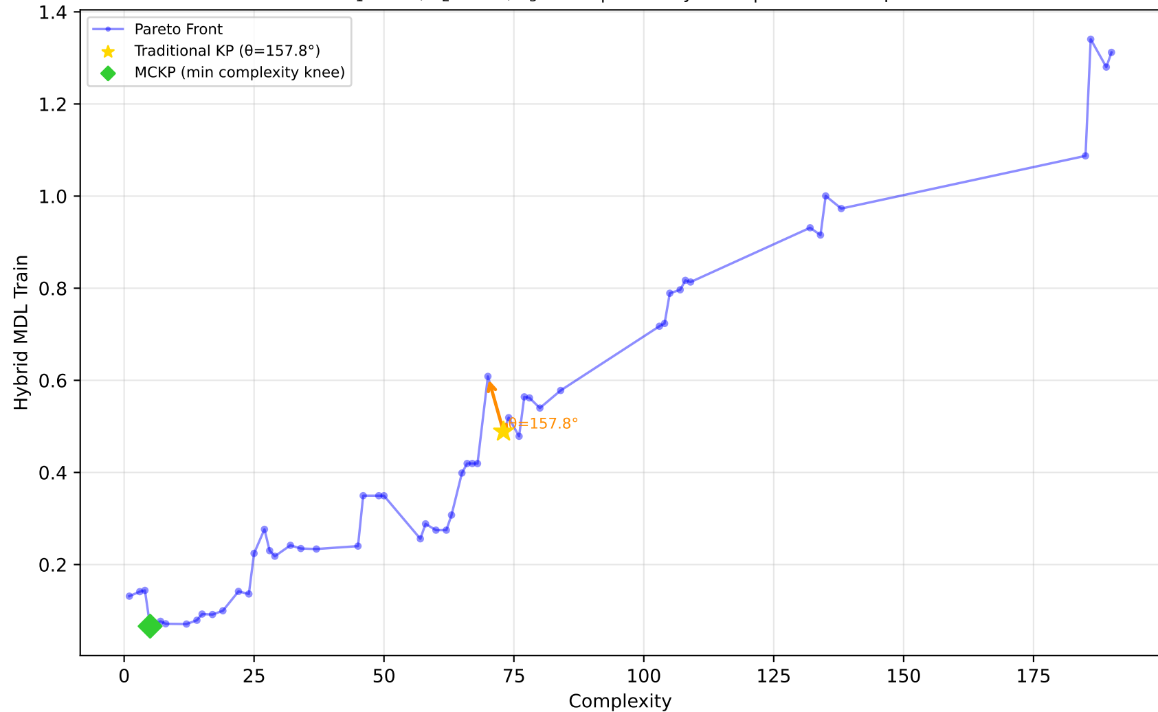
712_chscase_geyser1 - Run 19 - MVP - Hybrid MDL Train \lambda_1=0.20, \lambda_2=1.00, \lambda_3=1.00 | Difficulty: 0.58 | Method: mckp
