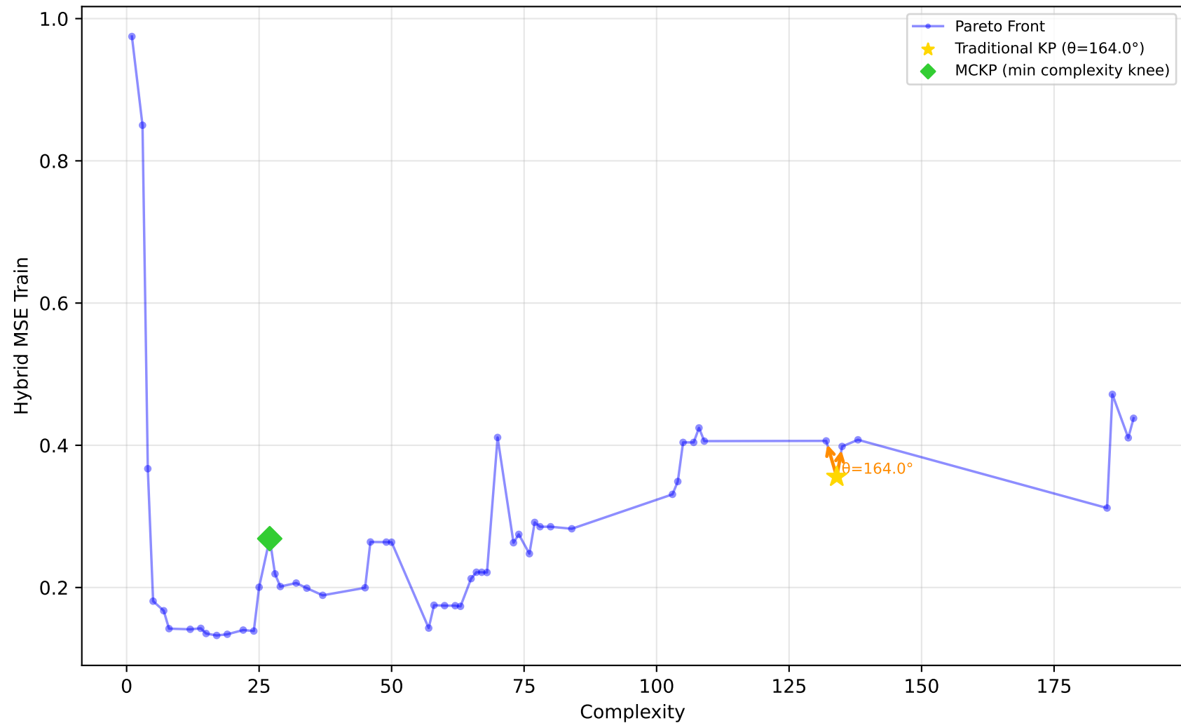
712_chscase_geyser1 - Run 19 - MVP - Hybrid MSE Train \lambda_1=0.20 , \lambda_2=1.00 , \lambda_3=1.00 | Difficulty: 0.58 | Method: mckp
