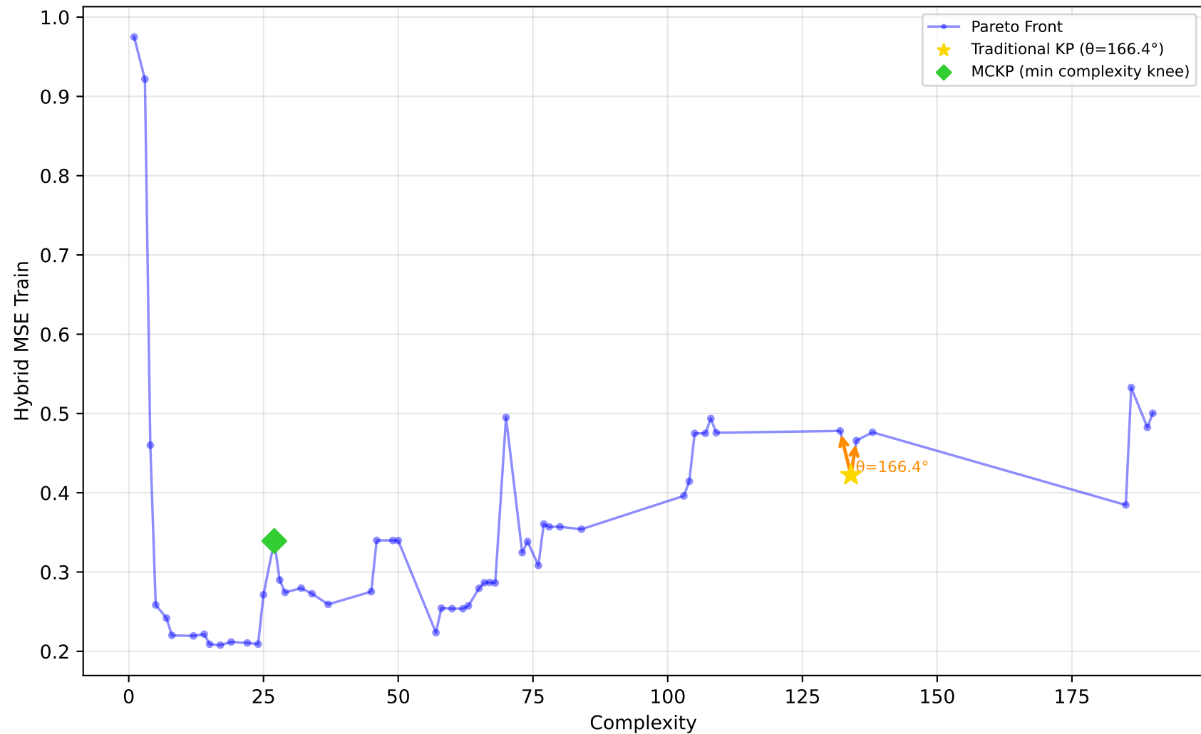
712_chscase_geyser1 - Run 19 - MVP - Hybrid MSE Train \lambda_1=1.00, \lambda_2=1.00, \lambda_3=1.00 | Difficulty: 0.58 | Method: mckp
