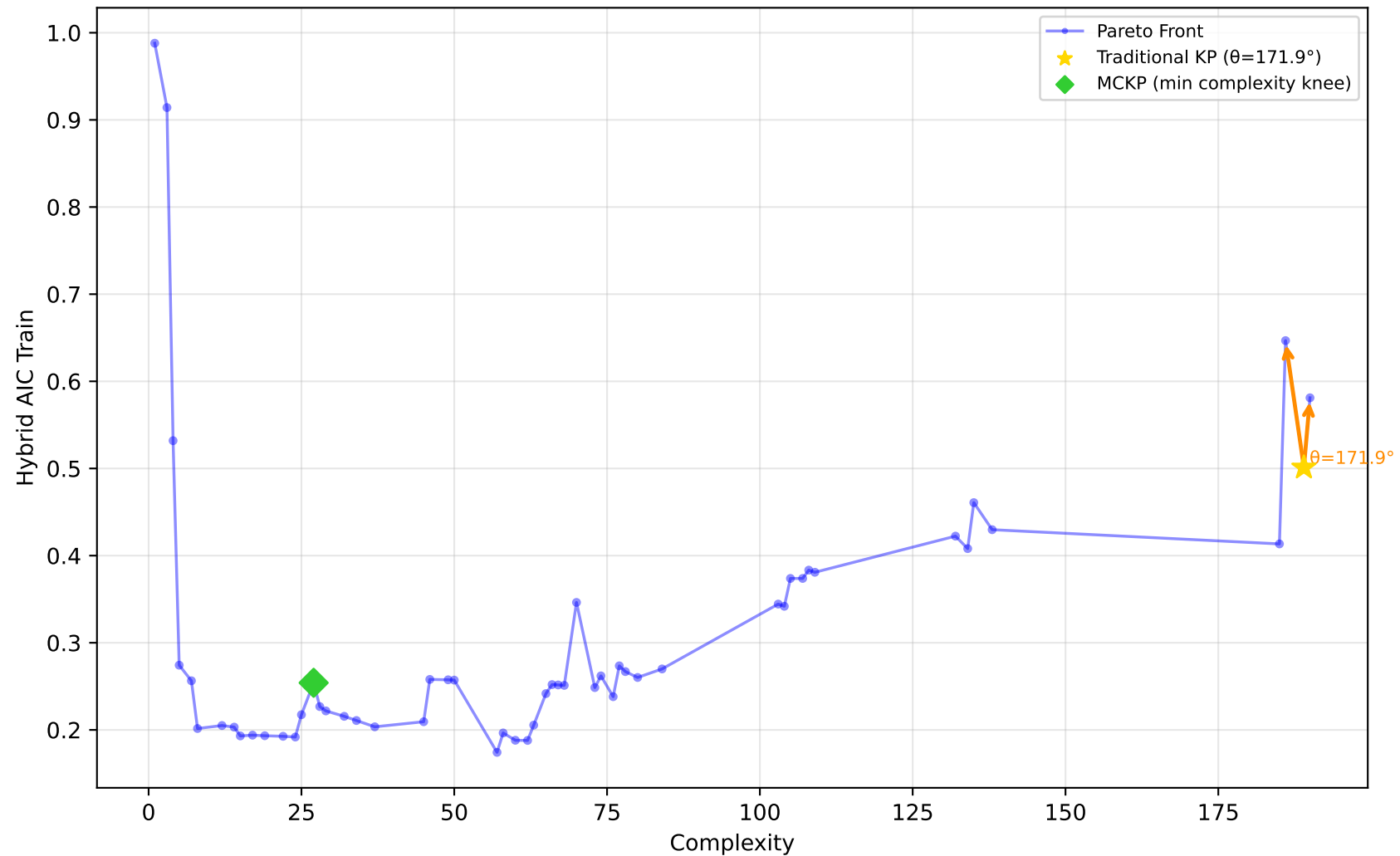
712_chscase_geyser1 - Run 19 - SVP - Hybrid AIC Train \lambda_1=0.00 , \lambda_2=1.00 , \lambda_3=1.00 | Difficulty: 0.58 | Method: mckp
