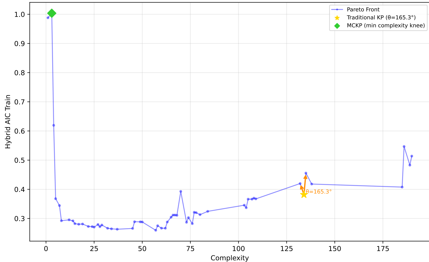
712_chscase_geyser1 - Run 19 - SVP - Hybrid AIC Train \lambda_1=1.00 , \lambda_2=1.00 , \lambda_3=0.00 | Difficulty: 0.58 | Method: mckp
