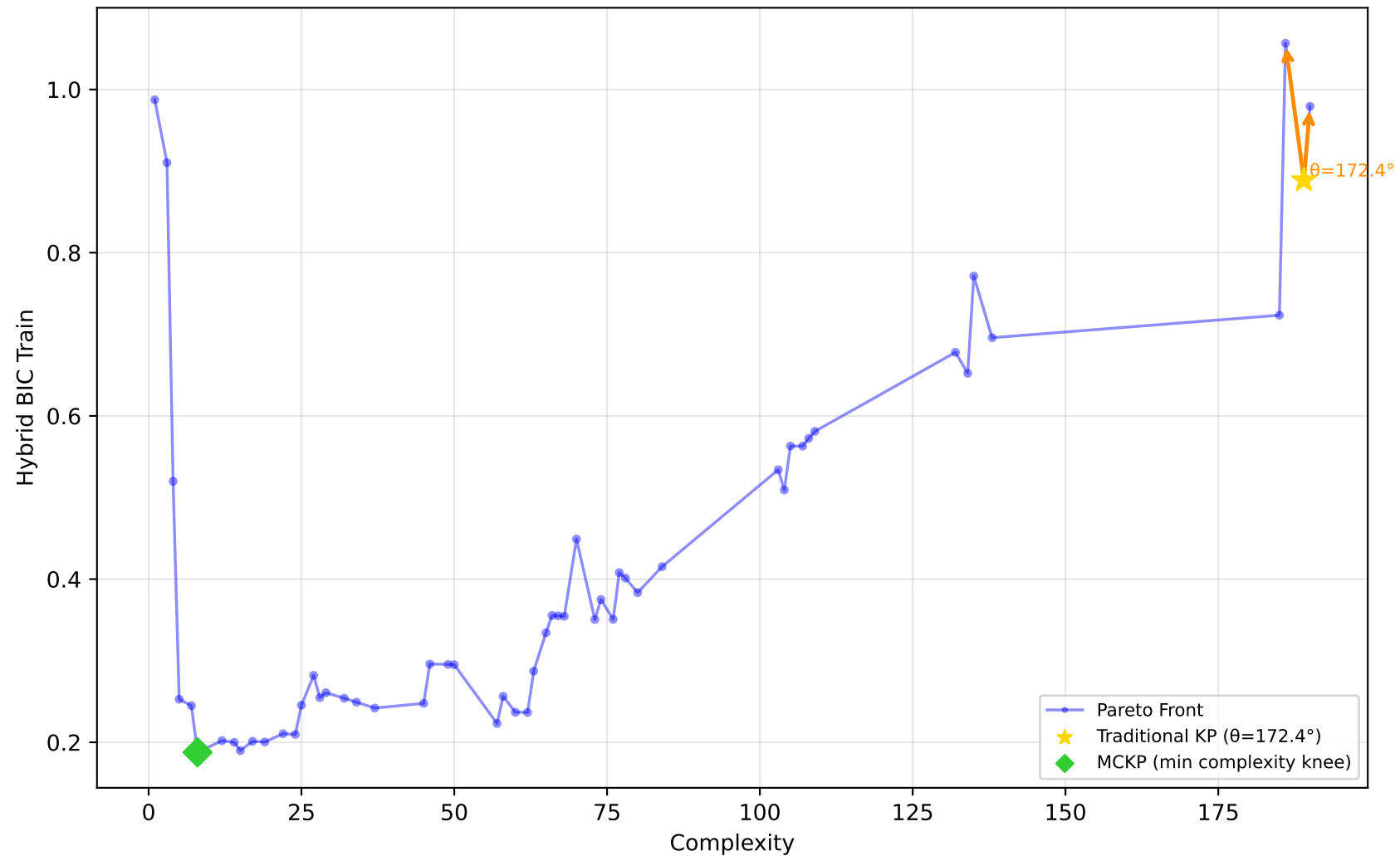
712_chscase_geyser1 - Run 19 - SVP - Hybrid BIC Train \lambda_1=0.00 , \lambda_2=1.00 , \lambda_3=1.00 | Difficulty: 0.58 | Method: mckp
