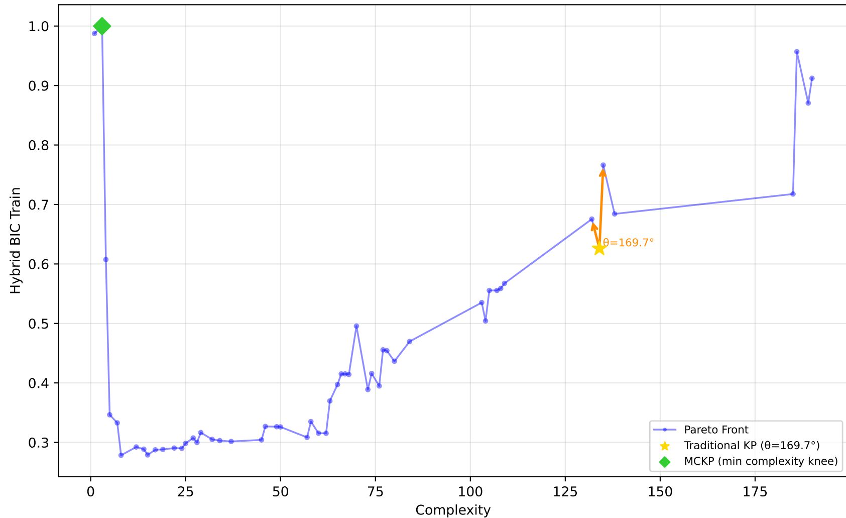
712_chscase_geyser1 - Run 19 - SVP - Hybrid BIC Train \lambda_1=1.00 , \lambda_2=1.00 , \lambda_3=0.00 | Difficulty: 0.58 | Method: mckp
