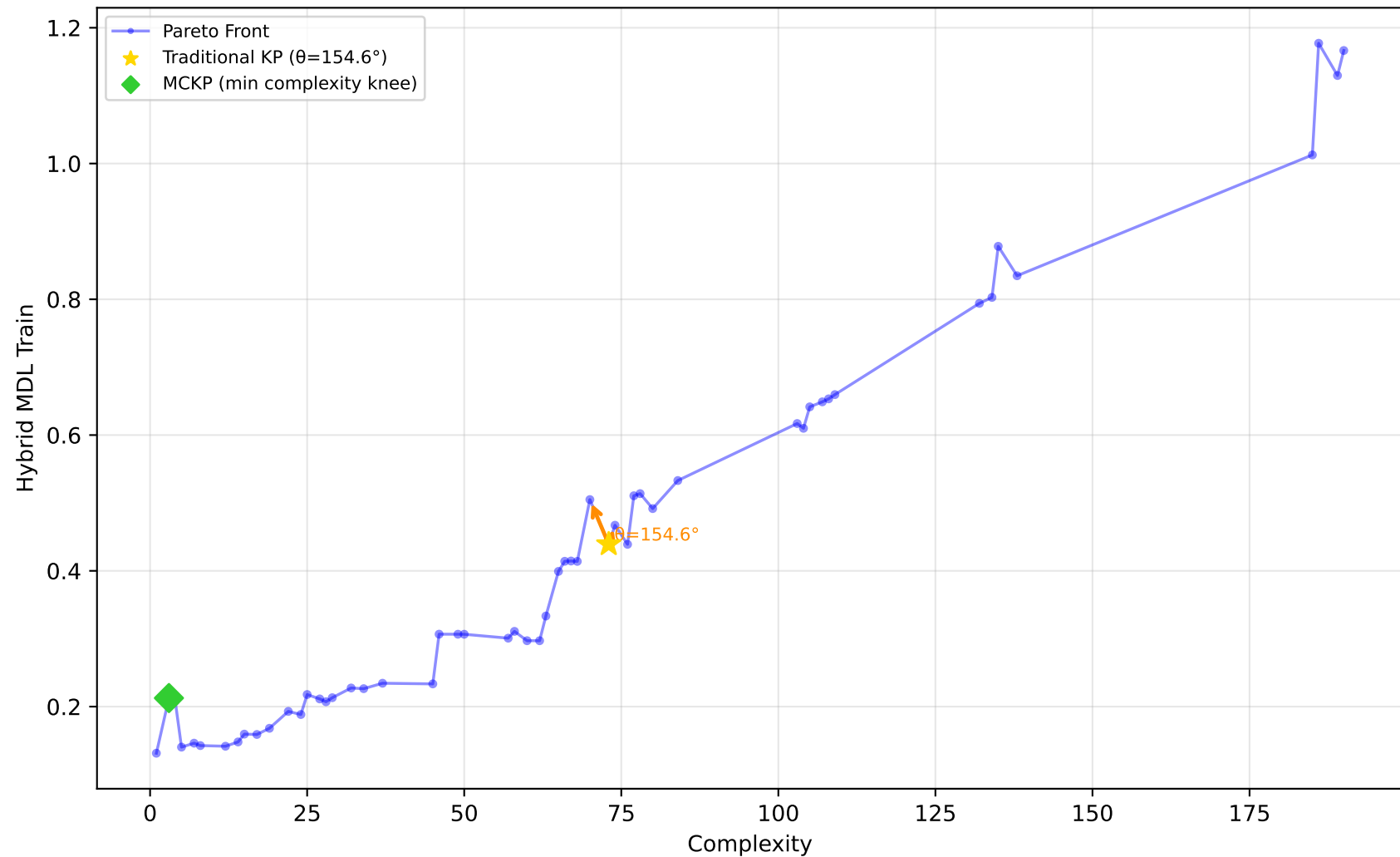
712_chscase_geyser1 - Run 19 - SVP - Hybrid MDL Train \lambda_1=1.00, \lambda_2=1.00, \lambda_3=0.00 | Difficulty: 0.58 | Method: mckp
