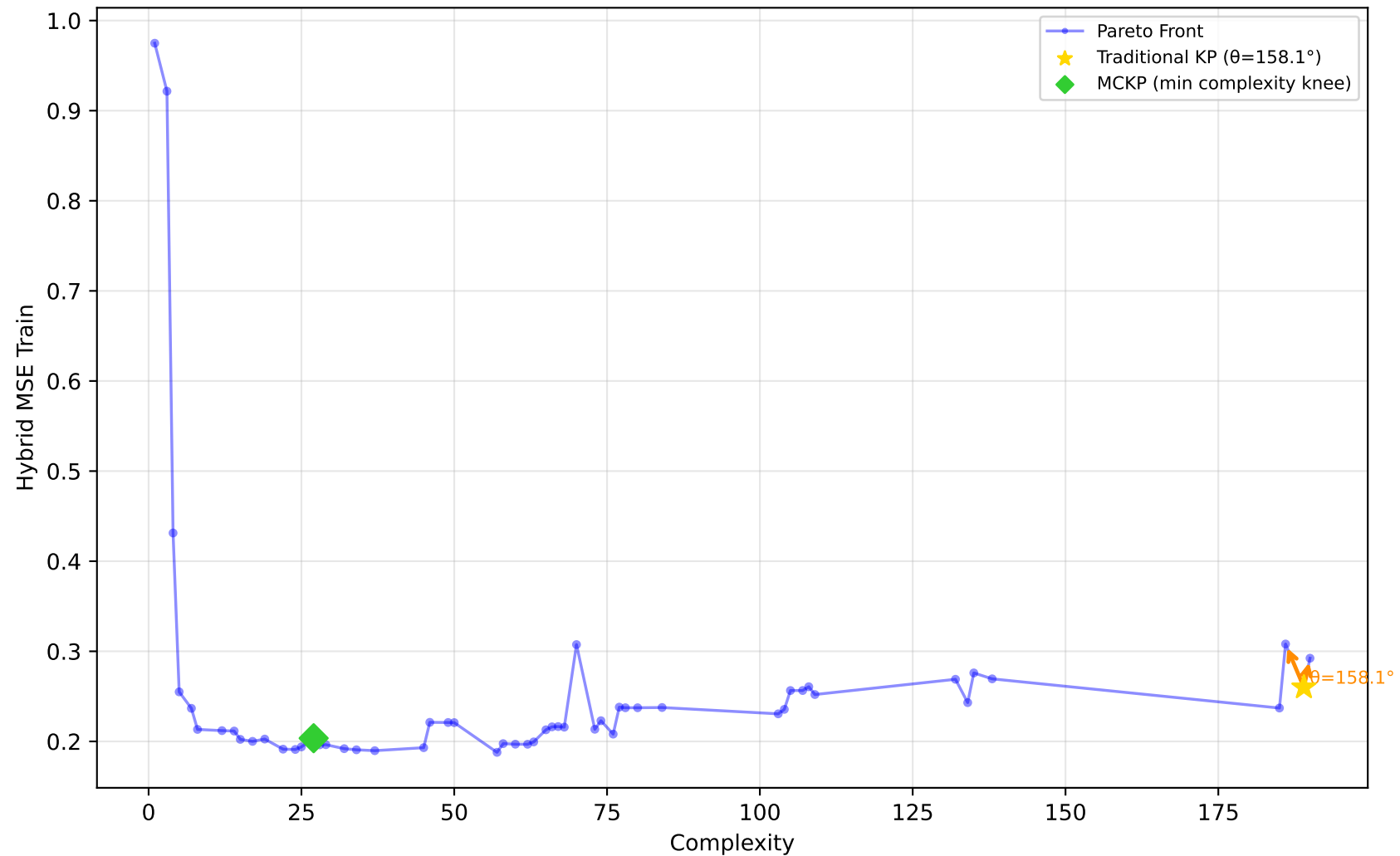
712_chscase_geyser1 - Run 19 - SVP - Hybrid MSE Train \lambda_1=1.00 , \lambda_2=1.00 , \lambda_3=0.00 | Difficulty: 0.58 | Method: mckp
