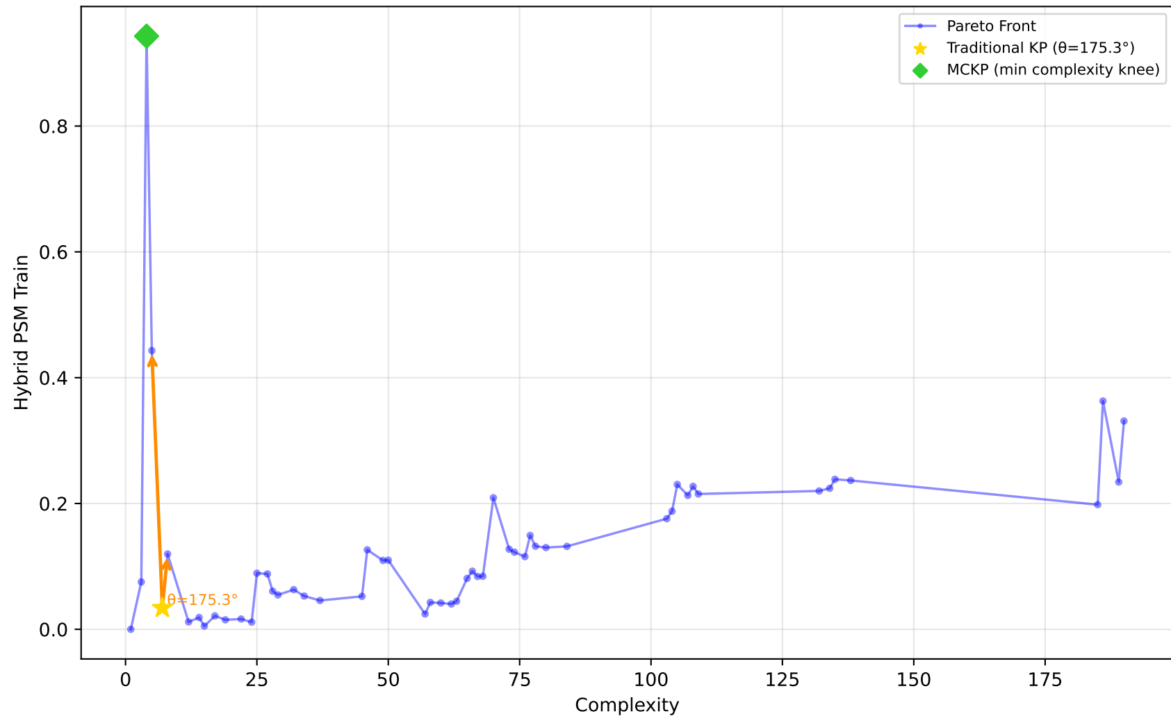
712_chscase_geyser1 - Run 19 - SVP - Hybrid PSM Train \lambda_1=0.00 , \lambda_2=1.00 , \lambda_3=1.00 | Difficulty: 0.58 | Method: mckp
