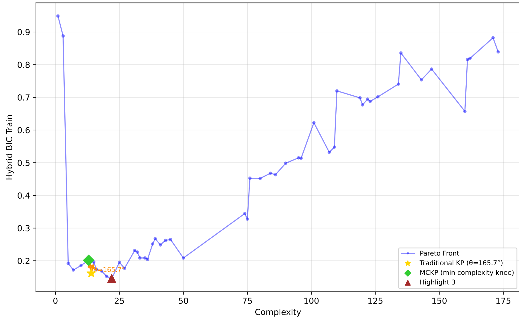
712_chscase_geyser1 - Run 1 - MVP - Hybrid BIC Train \lambda_1=0.20, \lambda_2=1.00, \lambda_3=1.00 | Difficulty: 1.00 | Method: hmr
