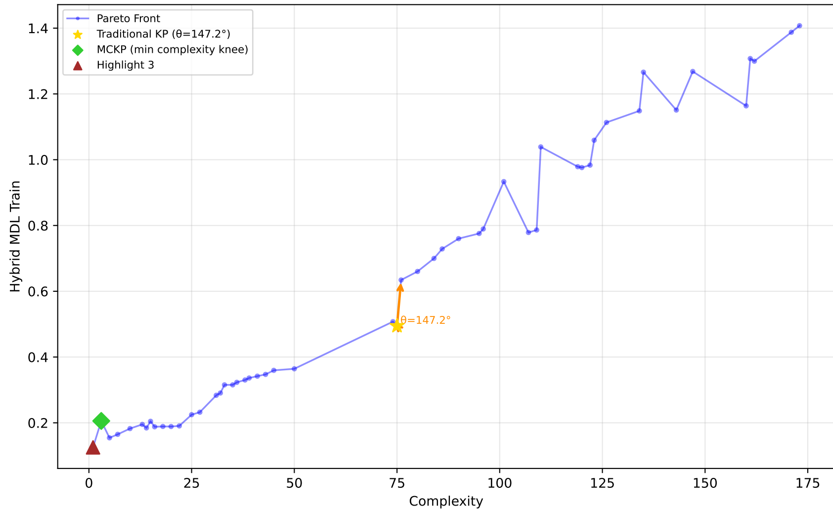
712_chscase_geyser1 - Run 1 - MVP - Hybrid MDL Train \lambda_1=1.00, \lambda_2=1.00, \lambda_3=1.00 | Difficulty: 1.00 | Method: hmr
